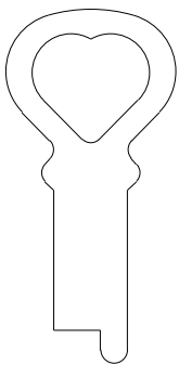
.050" - 1.3mm .300" - 7.6mm T45
