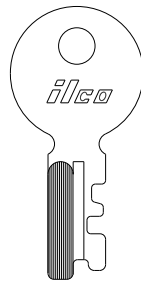
NICKEL SILVER .060" - 1.5mm .305" - 7.8mm 1326
