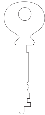
STEEL .065" - 1.65mm .266" - 6.76mm T75
